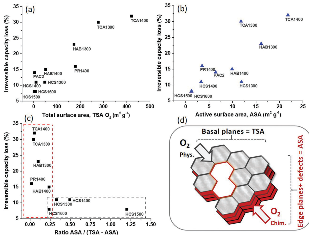
Fig. 3 Relationship between the 1st irreversible capacity loss and (a) total surface area ( TSA_{O_2} ), (b) active surface area ( ASA ), (c) ratio ASA/(TSA - ASA) . (d) Representation of hard carbon structure containing the active surface (edge planes and defects) and the basal planes surface ( TSA - ASA ).
