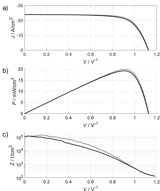
Fig. 4 Example of (a) JV curve forward scan (0 V \rightarrow V_{OC} , dotted line) and backward scan ( V_{OC} \rightarrow 0 V, full line) measured with a scan rate of 200 \text{ mV s}^{-1} ; (b) power density calculated from the respective JV curves demonstrating the efficiency of \sim 20\% ( 20 \text{ mW cm}^{-2} under standard 100 \text{ mW cm}^{-2} illumination); (c) slope of the JV curve (calculated from raw JV data with a smoothing filter). The slope is equivalent to the expected Z_{DC} = Z(\omega \rightarrow 0) . It should be considered that the measurement of the JV curve is also a dynamic measurement and might not reflect the exact Z_{DC} as a matter of principle.
