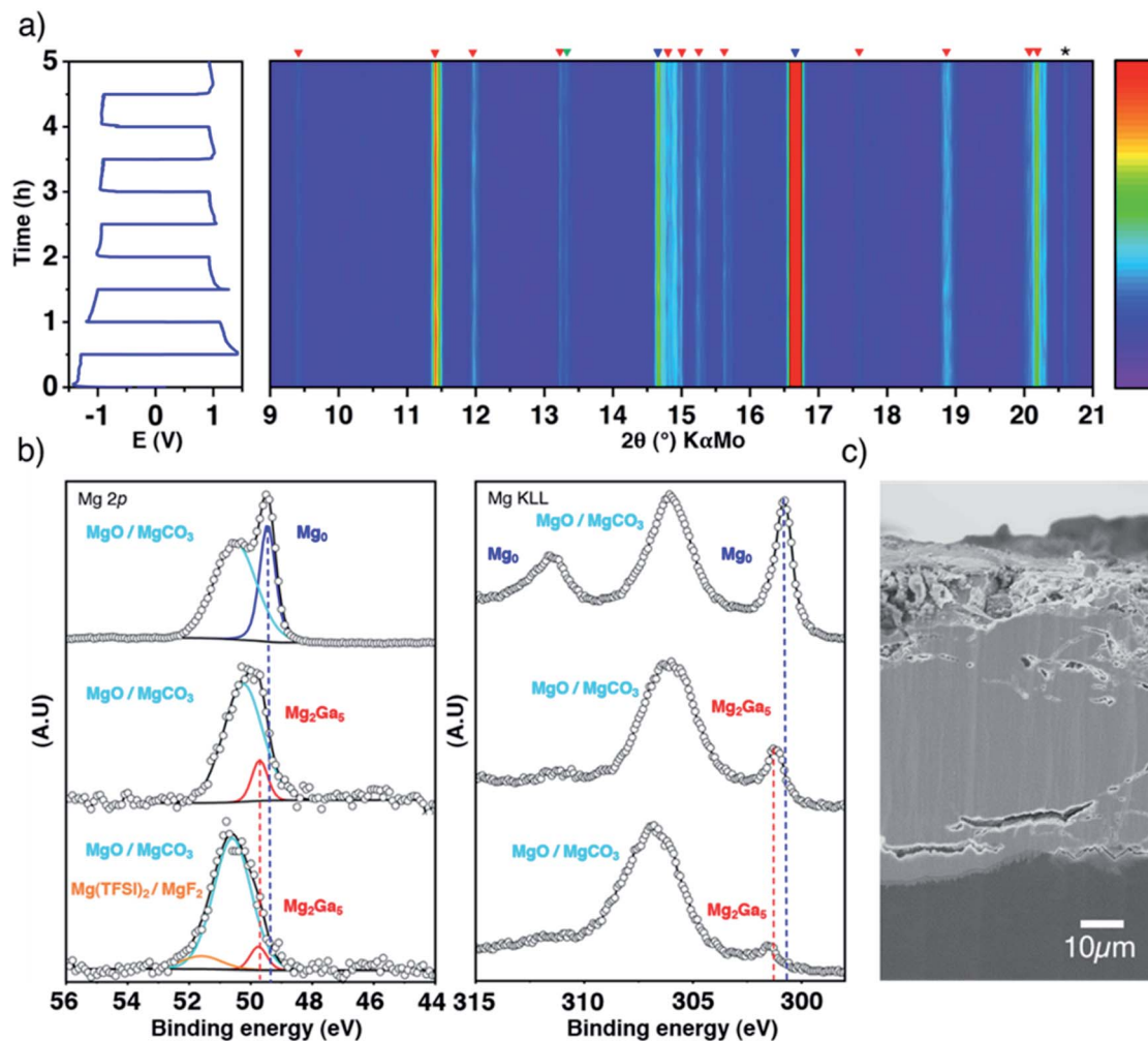
Fig. 3 Inside the coating evolution. Top-view representation of XRD patterns collected in situ in transmission mode during galvanostatic polarization measurements of a symmetric cell at 0.1 mA cm -2 , with blue, red and green markers for Mg, Mg 2 Ga 5 and Mg 2 Ga, respectively (a); XPS spectra (Mg 2p and Auger Mg KLL) of pristine Mg, Ga-coated Mg before and after 50 hours of plating/stripping, normalized by the most intense contribution (b); SEM cross-sectional image of the coated electrode after plating/stripping (c). Note that XRD acquisitions were performed at room temperature as the in situ cell does not allow working at 40 °C, even if the coating efficiency is not optimized at such temperature (Fig. S6†).
