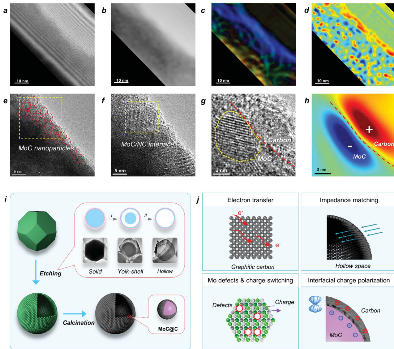
Fig. 5 (a) Hologram. (b) Reconstructed phase image. (c) Electric-fielded map. (d) Charge density map. (e) HR-TEM images. (f and g) MoC/NC hetero-interface. (h) Charge distribution on the MoC(-)/carbon(+) interface. (i) Two-step synthetic route and chemical etching mechanism (insert). (j) Illustration schemes of four electromagnetic wave attenuation mechanism.
