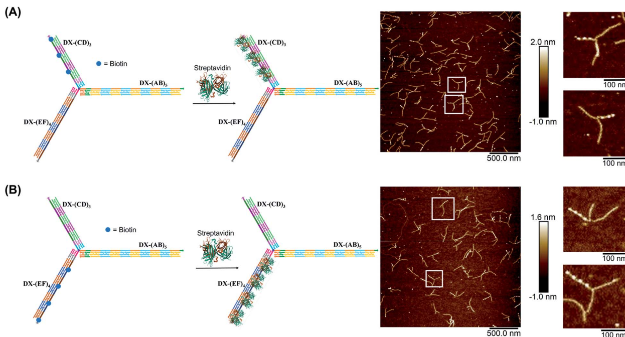
Fig. 4 AFM characterization of three-way DNA nanostructure patterned with periodic streptavidin proteins. Patterning of (A) DX-(CD) 3 arm and (B) DX-(EF) 4 arm. The bright dots in the AFM images correspond to the patterned streptavidin. The population of structures with exactly three (A) and four (B) streptavidin calculated from AFM images is 76% ( N = 186 ) and 77% ( N = 120 ), respectively. This percentage excludes the inter-connected structures resulting from sample deposition on the mica surface.
