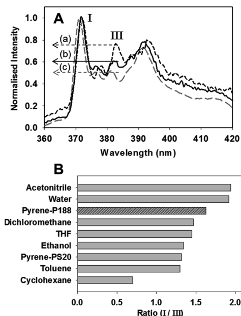
Fig. 12 Determination of microenvironment polarity within P 188 nanoparticles using pyrene as ratiometric emission probe. (A) Fluorescence spectra at rt of (a) pyrene in toluene (b) aqueous pyrene-P 188 (NP-pyrene-P 188 ) (c) pyrene in water, with the first (I) and third (III) identified. (B) Ratiometric values for pyrene emission first (I) and third (III) bands in organic solvents of varying polarity and water, aqueous P 188 and aqueous PS 20 .
