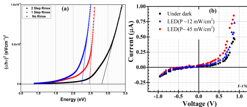
Fig. 7 (a) Variation of band gap with rinsing steps. (b) I - V characteristic curve for FTO/ \text{Cu}_2\text{O} /ZnO heterojunction cell grown on FTO substrate at pH-7.95. 101
