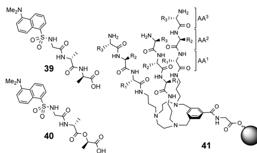
Fig. 15 Dansyl-labelled probes 39 and 40 and vancomycin mimetic combinatorial library 41 containing triazacyclopentane (TAC)-based tripeptides attached to O-glycine functionalised ArgoGel TM resin.
