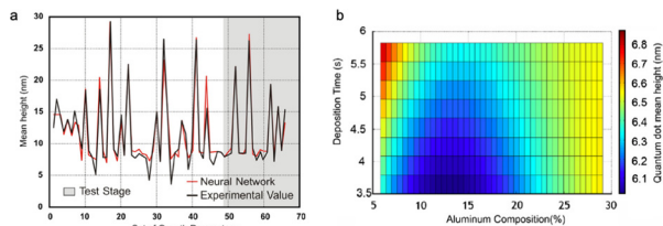
Fig. 6 A study of epitaxially-grown InAs QDs by Singulani et al. 111 (a) A comparison of an NN prediction for QD mean height with the obtained AFM experimental data. (b) A parameter map showing the output variable InAs QD height (nm) as a function of deposition time (s) and aluminium content of the InGaAlAs substrate. Reprinted from ref. 111, Copyright 2008, with permission from Elsevier.
