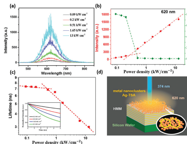
Fig. 5 (a) Emission spectra of the solid-state assembly of Ag-TSA MNCs over HMM under different pumping power densities of 374 nm pulsed pump excitation. (b) Emission intensity and line width as a function of the pumping power density showcasing the low threshold value (0.5 kW cm -2 ) of pump power density for the solid-state assembly of Ag-TSA MNCs over HMM. (c) Carrier lifetime as a function of the pumping power density for the solid-state assembly of Ag-TSA MNCs over HMM (inset: time-resolved photoluminescence (TRPL) measurements for the solid-state assembly of Ag-TSA MNCs over HMM under different pumping power densities of 374 nm pulsed pump excitation). (d) Schematic illustration of the stimulated emissions from the solid-state assembly of Ag-TSA MNCs over HMM under 374 nm pulsed pump excitation (Reproduced from ref. 63, with permission from [American Chemical Society]).
