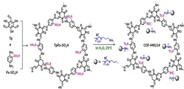
Scheme 16 The synthesis of TpPa- \text{SO}_3\text{H} and COF-HNU14. Reproduced with permission from ref. 36; copyright: 2020, ACS Sustainable Chemistry & Engineering.
