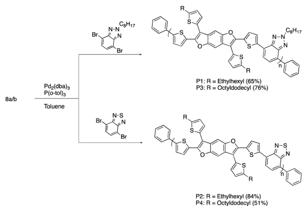
Scheme 2 Synthesis of D–A Copolymers P1–P4 .
