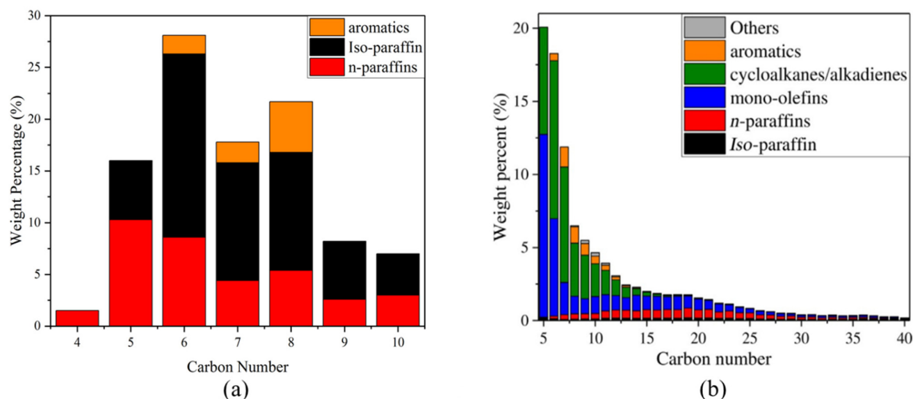
Fig. 17 (a) A typical naphtha composition (graph made based on the data obtained from ref. 251, (b) a typical plastic pyrolysis oil composition obtained from PE pyrolysis. Reproduced from ref. 252 with permission from Wiley-VCH, copyright 2020.
