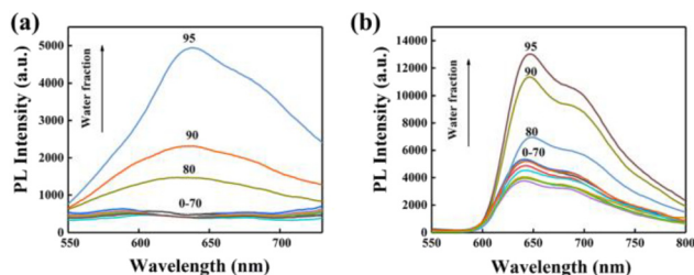
Fig. 2 PL spectra of Ir-1-N + (a) and Ir-2-N + (b) in \text{CH}_3\text{CN} – \text{H}_2\text{O} mixtures (complex concentration = 1.0 \times 10^{-5} M) with different water fractions (0–95% v/v) at room temperature.
