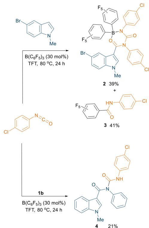
Scheme 4 Reactivity observed when using 5-bromo-1-methylindole with 4-chlorophenyl isocyanate to afford 2 and 3 (top). Amidation of 1b using 30 mol% B(C 6 F 5 ) 3 to afford 4 (bottom). All the reactions were carried out on a 0.1 mmol scale; yields reported are isolated yields.
