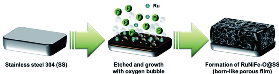
Fig. 88 Schematic of the formation mechanism of RuNiFe-O@SS electrocatalyst. Reproduced with permission from ref. 1298 Copyright RSC 2021.
