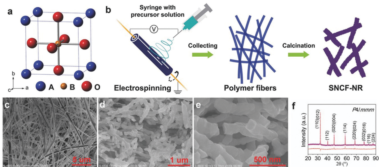
Fig. 32 (a) \text{ABO}_3 perovskite structure. (b) Schematic illustration of the preparation of SNCF-NR by electrospinning. (c) Scanning electron microscopy (SEM) image of as-spun precursory polymer nanofibers before calcination. (d and e) Low/high-magnification SEM images of SNCF-NR. (f) Refined XRD pattern of SNCF-NR. Observed (purple circles), calculated (red solid line), and differences (orange line, bottom) are presented. Reproduced with permission from ref. 619. Copyright Wiley 2017.
