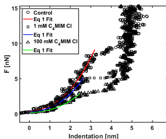
Fig. 5 Force curves on phospholipid bilayers interacting with [C 4 MIM][Cl] at different concentrations after equilibration time T_{eq} = 20 min. Typical examples of force vs. indentation (after contact) with fitting to eqn (1).
