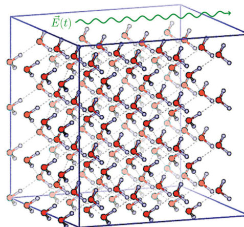
Fig. 1 Structure of proton-ordered ice VII model used in the simulations. The cubic supercell of side length 12.62 \text{ Å} contains 128 water molecules. Direction of the applied oscillating electric field is indicated by green arrow.
