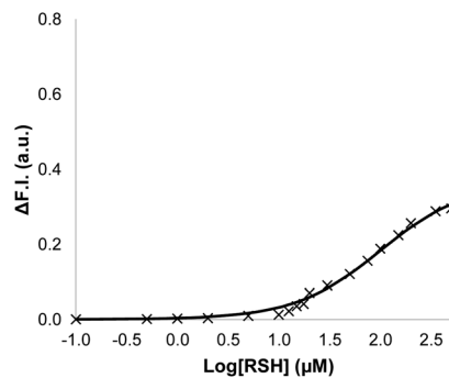
Fig. 7 Change in normalised fluorescence emission intensity at 440 \text{ nm} ( \lambda_{\text{exc}} = 365 \text{ nm} ) ( \Delta\text{F.I.} ) 360 \text{ min} after addition of different concentrations of benzyl thiol ( [\text{RSH}] ) to vesicles (DOPC, 1.0 \text{ mM} ) containing peptide substrate ( 250 \mu\text{M} ), caged papain ( 10 \mu\text{M} ) and 2 ( 10 \mu\text{M} , 1\% loading) in HEPES buffer ( \text{pH} = 7.2 ). The line is the best fit to an isotherm for equilibrium formation of a 1 : 1 adduct between the thiol and 2 .
