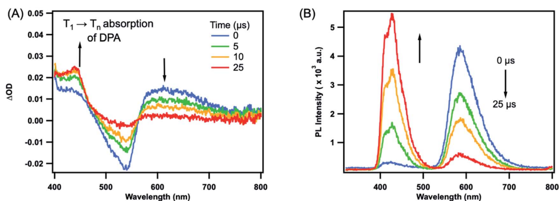
Fig. 3 Transient absorption difference spectra (A), and time-resolved photoluminescence spectra (B) of Zr( Mes PDP Ph ) 2 ( OD_{514 \text{ nm}} = 0.4 ) and 0.25 \text{ mM} DPA in deaerated THF at several delay times following 514 \text{ nm} pulsed laser excitation ( \sim 2 \text{ mJ} per pulse) with delay times indicated.
