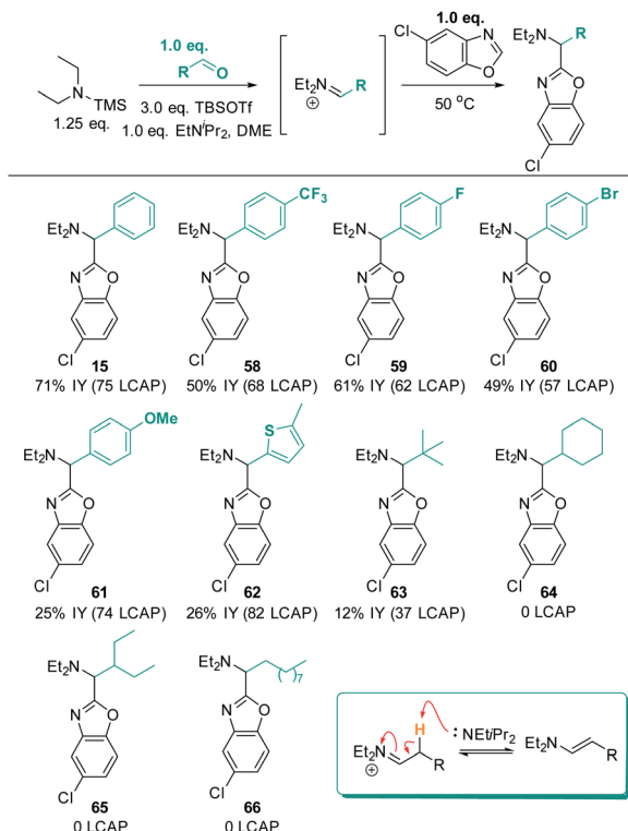
Scheme 16 Aldehyde scope. Conditions: azole (1.0 eq.), TBSOTf (0.416 mL, 1.813 mmol, 3.0 eq.), \text{TMS-NEt}_2 (1.25 eq.), \text{PhCHO} (1.0 equiv.), \text{EtN}^i\text{Pr}_2 (1.0 equiv.), \text{N}_2 , 50 °C, 18 h.
