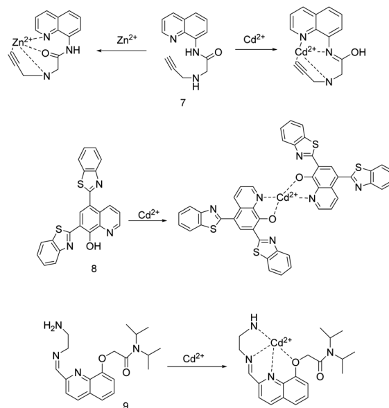
Fig. 3 Proposed binding mode of probes 7 to 9 with Cd 2+ .
