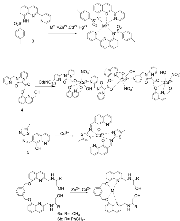
Fig. 2 Proposed binding mode of probes 3 to 6 with Cd 2+ .
