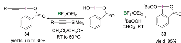
Scheme 13 Transformation of benzoiodoxolone into the corresponding alkylperoxyiodinane 33 and alkynyl derivative 34.
