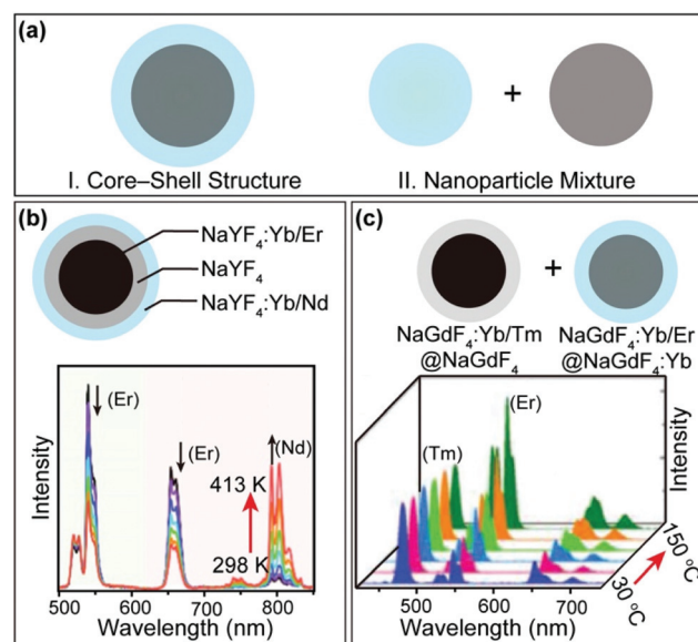
Fig. 5 (a) Schematic illustration of integrating upconversion components displaying distinct temperature dependence of luminescence. (b) Emission spectra of \text{NaYF}_4:\text{Yb}/\text{Nd} (20/6%)@ \text{NaYF}_4 @ \text{NaYF}_4:\text{Yb}/\text{Er} (20/0.5%) nanorods in the temperature range of 298–413 K. Adapted with permission from ref. 89. Copyright 2019, American Chemical Society. (c) Emission spectra of \text{NaGdF}_4:\text{Yb}/\text{Er} @ \text{NaGdF}_4 nanoparticles mixed with \text{NaGdF}_4:\text{Yb}/\text{Er} @ \text{NaGdF}_4:\text{Yb} in the temperature range of 30–150 °C. Adapted with permission from ref. 90. Copyright 2019, Wiley-VCH.
