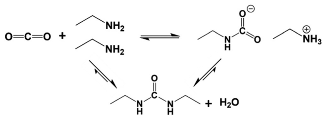
Fig. 21 Relationship between formation of carbamate and urea species during CO 2 adsorption-desorption under dry conditions. Adapted with permission from ref. 123. Copyright (2010) American Chemical Society.
