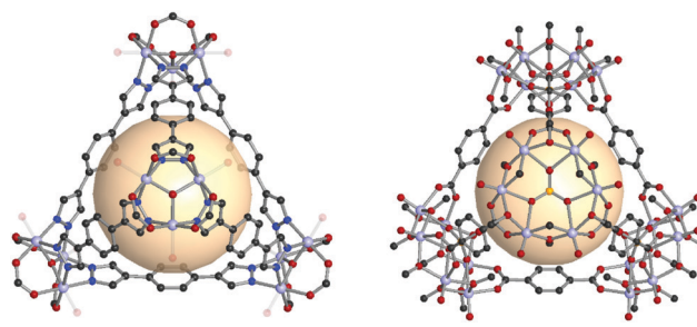
Fig. 9 Structural illustration of [\text{V}_3\text{O}_2(\text{OH})_2(\text{COOH})_3]_4(\text{A18})_6 (left) 56 and VMOP-11, [\text{V}_6\text{O}_6(\text{OCH}_3)_9(\text{SO}_4)]_4(\text{A1})_6 (right). 57
