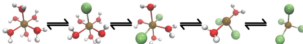
Fig. 1 A schematic of the ligand exchange reaction of [\text{Co}(\text{H}_2\text{O})_6]^{2+} investigated in this work. The equilibrium can be affected by a sudden temperature (e.g. T-jump) or concentration change, leading to structural interconversion via ligand exchange with \text{Cl}^- ions.
