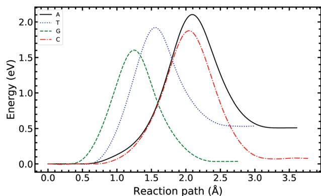
Fig. 6 Minimum energy path of the intra-base transfer reaction of the canonical to the tautomeric state of adenine, thymine, guanidine, and cytosine base pairs. The ML-NEB uncertainty is below the line thickness and not displayed.
