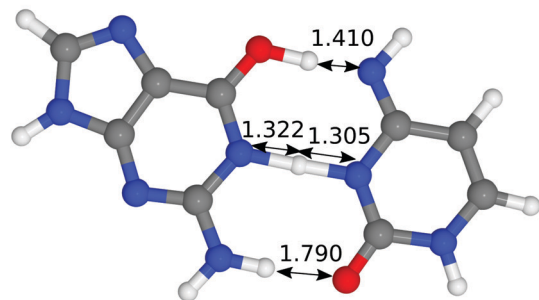
(b) Guanine-Cytosine transition state
