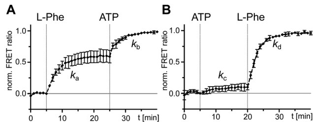
Fig. 3 Probing separated addition of ATP and L-Phe with holo-A-PCP sensor. Shown are normalized time-courses of the FRET ratio. At the indicated time points, the holo-A-PCP sensor (0.3 μM) was exposed to (A) first L-Phe (2 mM) and then ATP (2 mM) or (B) first ATP (2 mM) and then L-Phe (2 mM). The rates of the marked increases of the FRET ratio were fitted to k_a = (4.5 \pm 0.3) \times 10^{-3} \text{ s}^{-1} , k_b = (5.7 \pm 0.4) \times 10^{-3} \text{ s}^{-1} , k_c = (3.5 \pm 1.4) \times 10^{-3} \text{ s}^{-1} and k_d = (5.4 \pm 0.1) \times 10^{-3} \text{ s}^{-1} . FRET signals were determined as ratios I_a/I_d (intensity acceptor/intensity donor) and normalized between 0 and 1 using the signal at the time point before substrate addition and the respective maximum of the measurement series as reference points. Shown are the mean \pm SD of three independent measurements each consisting of three technical replicates.
