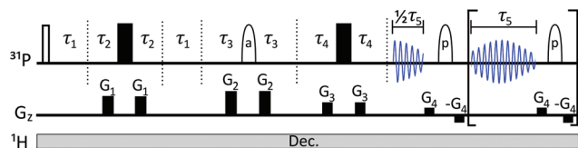
Fig. 3 The pulse sequence is effectively a combination of SAPPHIRE 20 and semi-RT 23 sequences, with one additional delay \tau_2 . G_z describes gradient pulses. Filled rectangles stand for 180° hard pulses, unfilled rectangle for 90° hard pulse. Ellipses denote 180° RSNOB soft pulses for (a) active spins (that will be detected) and (p) for passive spins. Hence, prior knowledge of the spectral position of passive and active spins is required. Following the semi-RT example, 23 Tycko-7/MLEV-4 supercycle is used for passive spin RSNOB pulses. Explanations for delays \tau_1 – \tau_5 and further details are given in ESI†.
