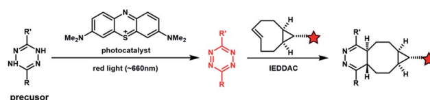
Fig. 4 Photocatalytic activation of the IEDDAC reaction.
