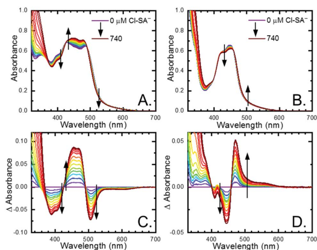
Fig. 4 UV-vis absorption spectra of (A) Ru-Dtb and (B) Ru-Bpz (~25 \mu\text{M} ) upon the addition of 0 to 740 \mu\text{M} Cl-SA • . Difference spectra calculated by subtracting the absorption spectra at no Cl-SA • from the spectra with Cl-SA • present for (C) Ru-Dtb and (D) Ru-Bpz . Arrows indicate the spectral changes upon Cl-SA • addition.
