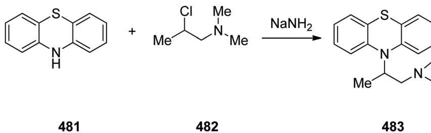
Scheme 68 Synthesis of promethazine 483.
