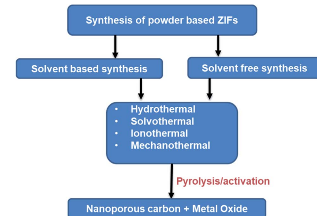
Fig. 5 Summary of the synthetic methods to convert ZIFs to ZIF-derived NPC and MO materials.
