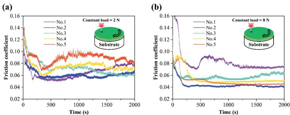
Fig. 7 The friction coefficient of \text{MoS}_2/\text{Ti} - \text{MoS}_2/\text{Si} multilayer nanocomposite coatings under the constant loads of 2 N (a) and 8 N (b), respectively.
