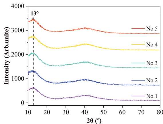
Fig. 5 XRD pattern of MoS 2 /Ti–MoS 2 /Si multilayer nanocomposite coatings.
