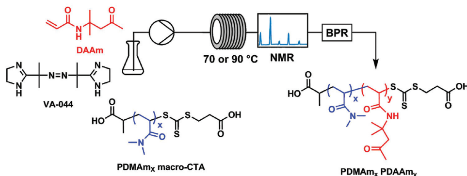
Fig. 1 Continuous-flow reactor configuration and chemical structures for the synthesis of polydimethyl acrylamide (PDMAm)- b -polydiacetone acrylamide (PDAAm) nano-objects.
