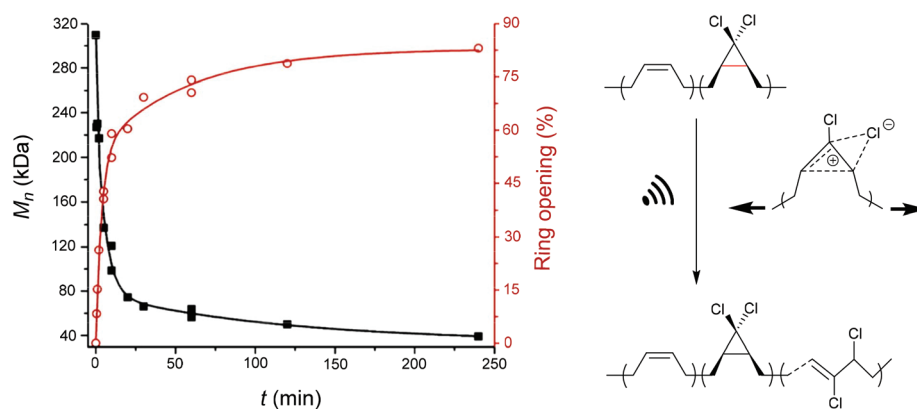
Fig. 4 Ultrasonication of gDCC-PB copolymer leads to ring-opened 2,3-dichloroalkenes (O) with simultaneously decreasing M_n (■). Adapted with permission from ref. 120. Copyright 2009 American Chemical Society.
