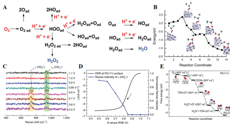
Fig. 9 (A) Schematic illustration of the possible ORR pathways. Reproduced with permission from ref. 166. Copyright 2019, Wiley-Blackwell. (B) Minimum-energy paths on the Pd(111) surface in the presence of hydrated proton. Reproduced with permission from ref. 167. Copyright 2013, American Chemical Society. (C) In situ EC-SERS spectra of the ORR system at a Pt(111) electrode surface in a 0.1 M HClO 4 solution saturated with O 2 . (D) Normalized EC-SERS intensities of the stretching mode of O–OH around 732 cm -1 at different potentials. (E) The proposed ORR mechanism at Pt(111) surfaces in 0.1 M HClO 4 solution and relevant Gibbs free energy (eV). Reproduced with permission from ref. 169. Copyright 2018, Springer Nature.
