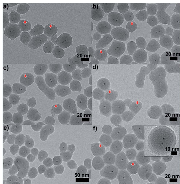
Fig. 9 TEM images of Au 25 @SiO 2 materials calcined at (a) 250 °C, (b) 350 °C, (c) 450 °C, (d) 550 °C, and (e) and (f) 650 °C (inset: enlarged image). Reproduced with permission of the Royal Society of Chemistry. 100
