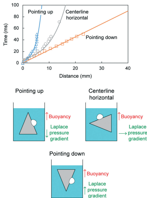
Fig. 21 Effect of cone orientation on air bubble movement (adapted from ref. 19). Distance traveled by air bubbles is shown as a function of time.
