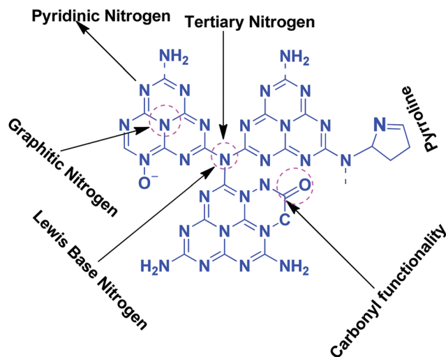
Scheme 5 Different types of N and O functionalities present in g-C 3 N 4 .
