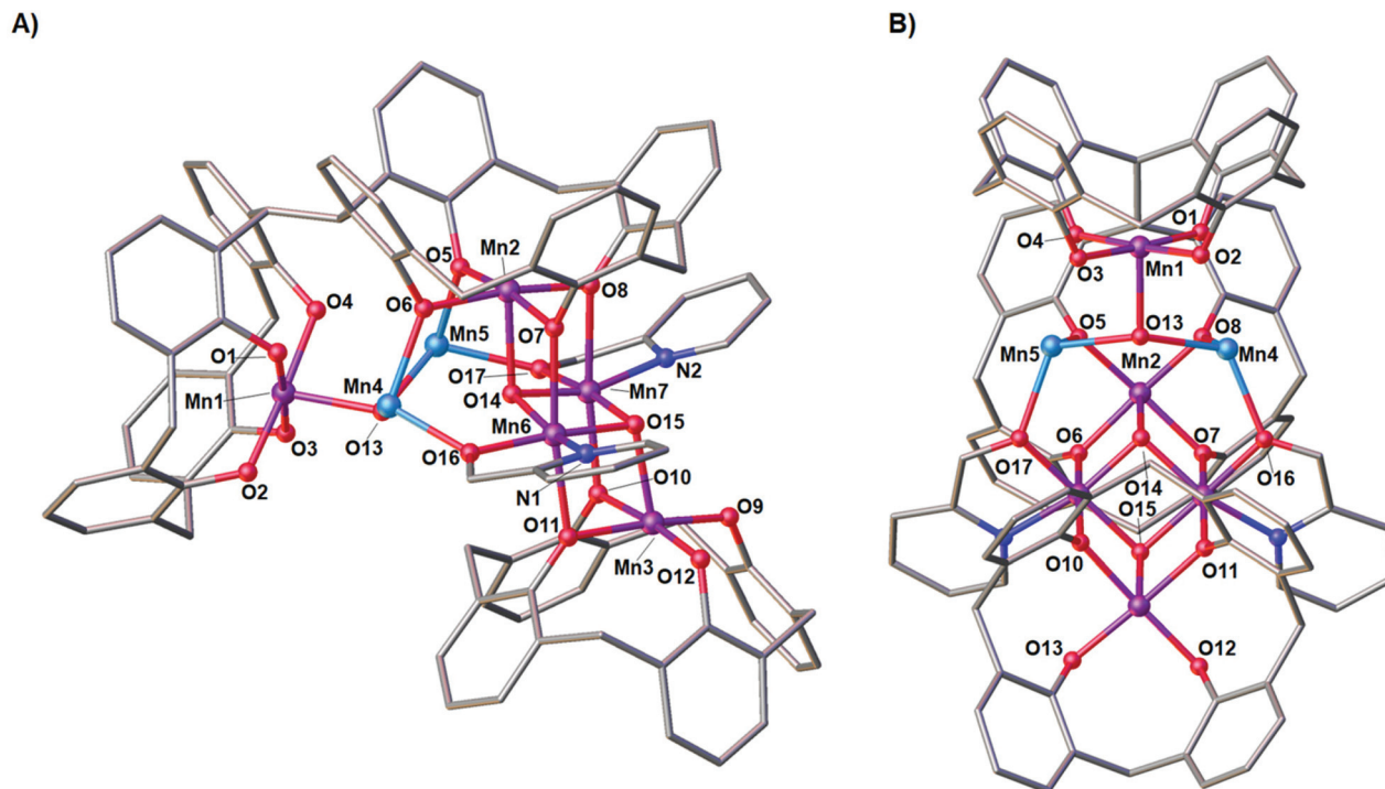
Fig. 3 Side (A) and orthogonal (B) views of the partial single crystal X-ray structure of the asymmetric unit in 6 . Selected labels have been added according to discussion. Colour code C – grey, O – red, N – royal blue, Mn II – pale blue, Mn III – purple. Hydrogen atoms, t Bu groups, ligated solvent molecules and co-crystallised solvent/anions omitted for clarity. Figures not to scale.
