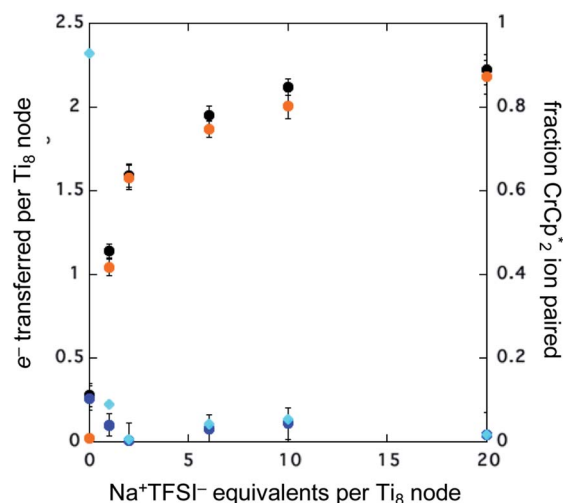
Fig. 3 Reduction of MIL-125 with 6 equiv. \text{CrCp}_2^* and 0–20 equiv. \text{Na}^+ in d_8 -THF + \text{CD}_3\text{CN} 4 : 1 v/v. Plot of e^- transferred to MIL-125 (left axis) and fraction of \text{CrCp}_2^* ion-paired in reduced MIL-125 (right axis) versus equiv. \text{NaTFSI} added. Orange circles: equiv. \text{Na}^+ associated with the reduced MIL-125, derived from the \text{CrCp}_2^{0/+} chemical shift. Blue circles: equiv. \text{CrCp}_2^* that are associated with the reduced MIL-125, derived from the change in integration of the \text{CrCp}_2^{0/+} resonance upon mixing with MIL-125. Black circles: total extent of reduction (sum of blue and orange). Light blue diamonds represent the fraction of the reduced MIL-125 that is associated with \text{CrCp}_2^* .
