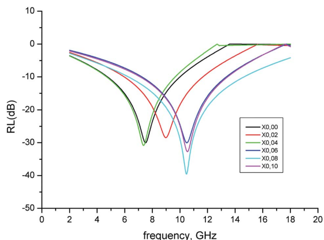
Fig. 9 RL spectra of \text{Ni}_{0.4}\text{Cu}_{0.2}\text{Zn}_{0.4}\text{La}_x\text{Y}_x\text{Fe}_{2-x}\text{O}_4 ( x = 0.00 - 0.10 ) NSFs.
