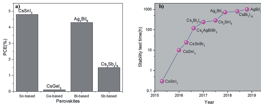
Fig. 2 (a) Highest PCE of devices based on different inorganic lead-free perovskite materials reported to date (classified by element). (b) Stability test time evolution of inorganic lead-free perovskites.
