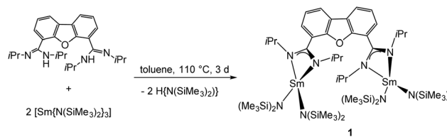
Scheme 4 Synthesis of 1 .
