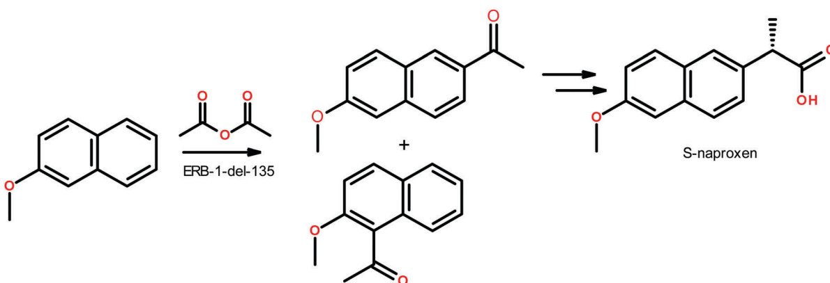
Scheme 4 Acylation of 2-methoxynaphthalene with acetic anhydride and illustration of the route to S-naproxen.
