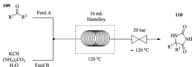
Fig. 15 Continuous flow synthesis of hydantoins.
