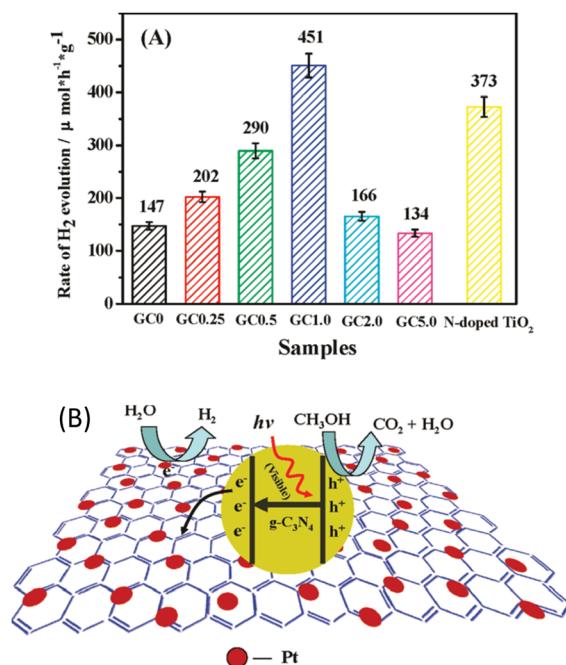
Fig. 9 (A) Comparison of the photocatalytic activities of samples with different loading amounts of graphene on g\text{-C}_3\text{N}_4 polymers, (B) proposed mechanism for the enhanced electron transfer process of the graphene/ g\text{-C}_3\text{N}_4 polymers. Reprinted with permission from ref. 48. Copyright 2011, American Chemical Society.
