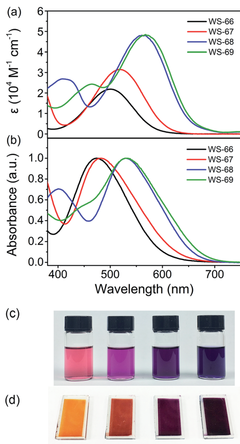
Fig. 2 Absorption spectra of dyes WS-66 , WS-67 , WS-68 and WS-69 in CH 2 Cl 2 (a) and on 3 \mu m TiO 2 films (b). Photographs of dyes WS-66 , WS-67 , WS-68 and WS-69 (from left to right) in solution (c) and on TiO 2 films (d).
